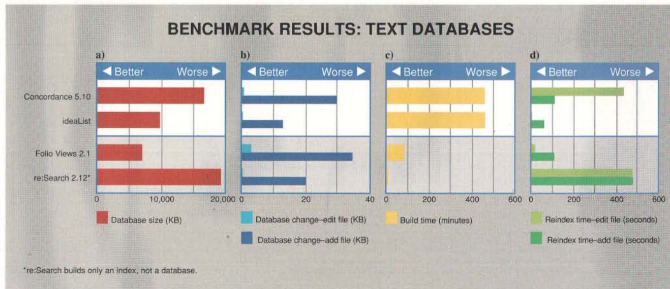
Figure 2: Benchmarks for text libraries (bottom two) and free-form database managers (top two) are similar to those we used for file-indexing packages, but these text management packages build and modify entire databases, not just indexes.
